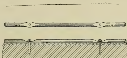
Courtesy of The Standard Paint Co. Fig. 142.—Wire Roofing Fastener.
